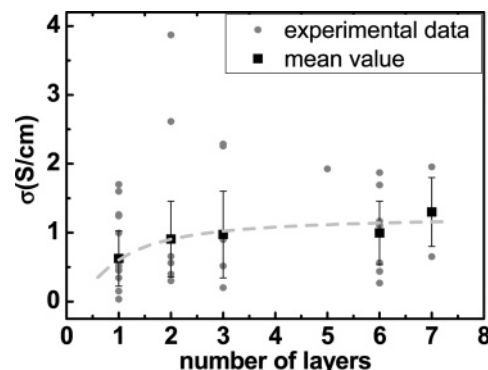
Figure 6. (a) Plot of the mean volume conductivity (measured under ambient conditions) as a function of the number of layers within fully reduced GO sheets. The gray dashed line has been drawn as a guide for the eye.
